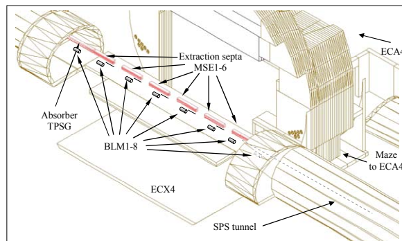
Figure 1: Tunnel, platform, shielding and beam loss monitor layout in the extraction region.
